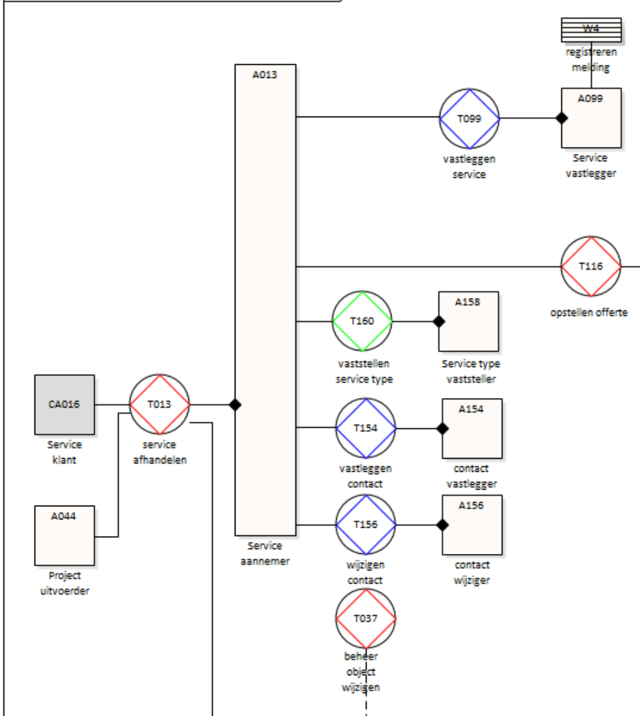
Organisation Construction Diagram OCD Afhandelen service order
